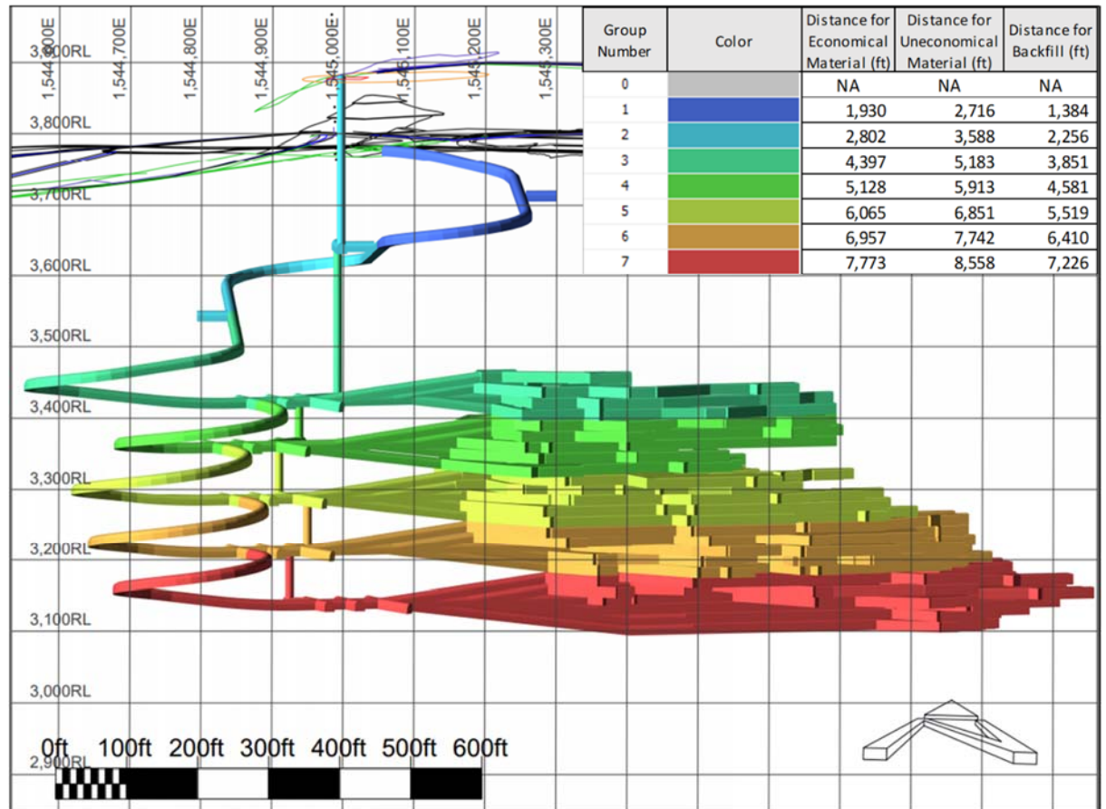
Figure 16-27: Distances for the Ton*Mile Calculation
