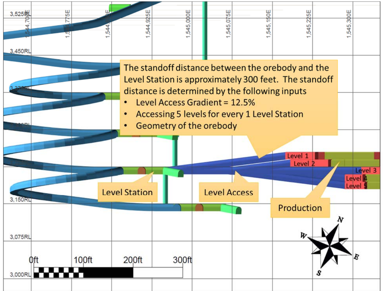
Figure 16-18: Level Access Layout (Looking North)
