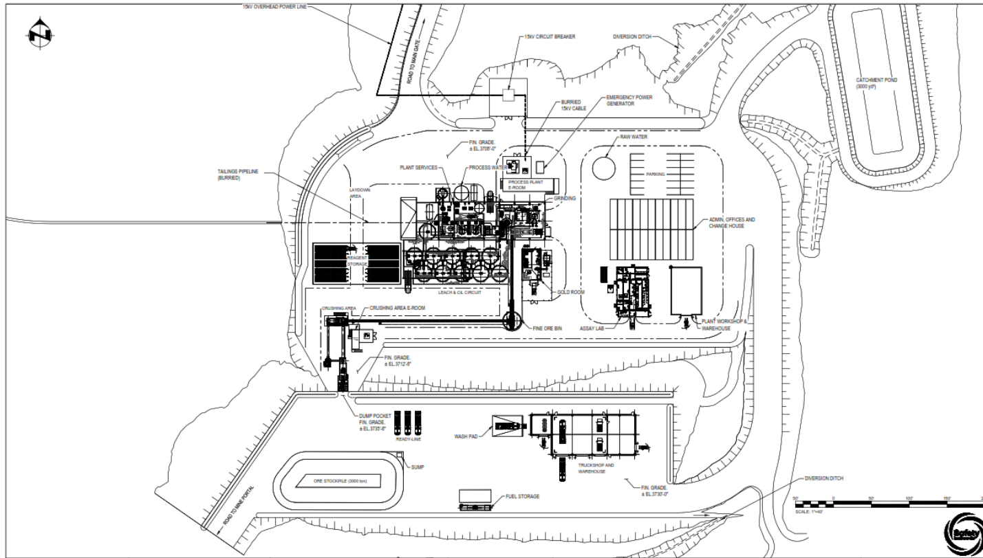
Figure 17-2: Proposed Plant Site Layout
