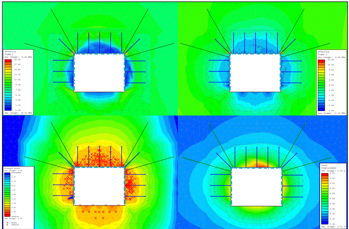
Figure 16-15: Modeling Results for Undercut B; a) Major Principal Stress, S1; b) Minor Principal Stress, S3; c) Strength Factor, SF; d) Displacements, D.
