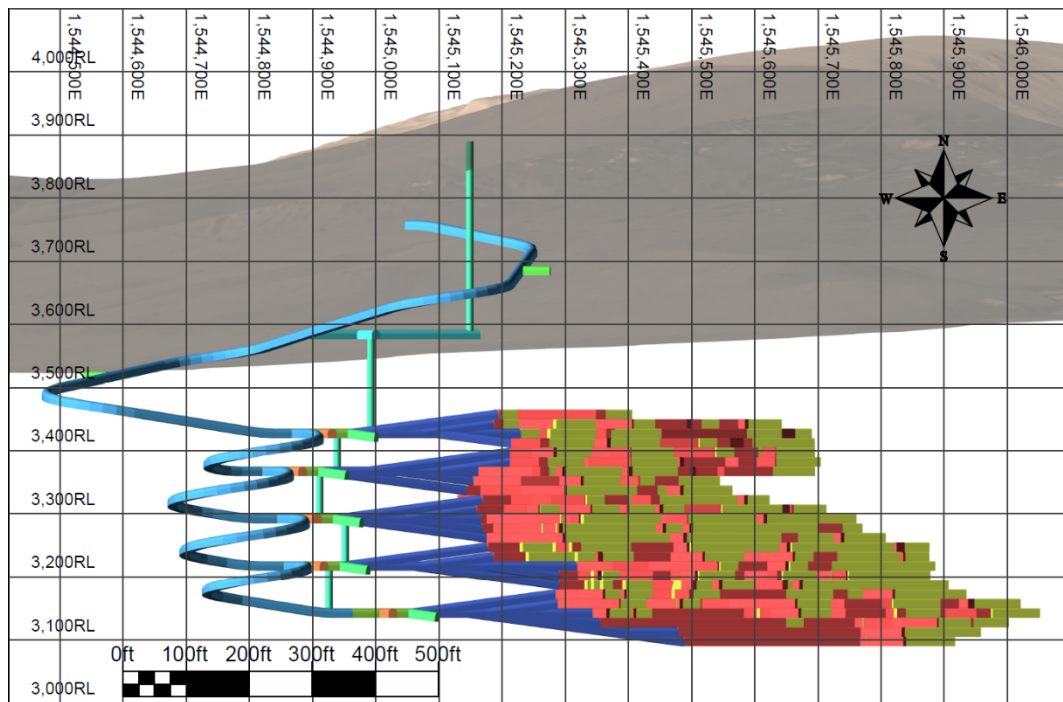
Figure 16-1: Grassy Mountain Mine Cross Section Looking North
