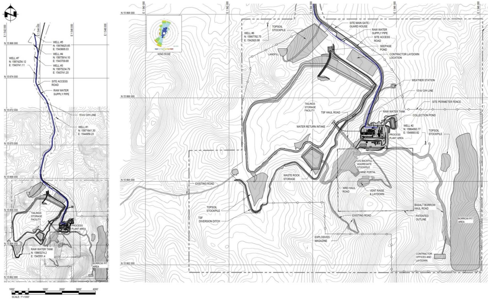
Figure 18-1: Proposed Infrastructure Layout Plan
