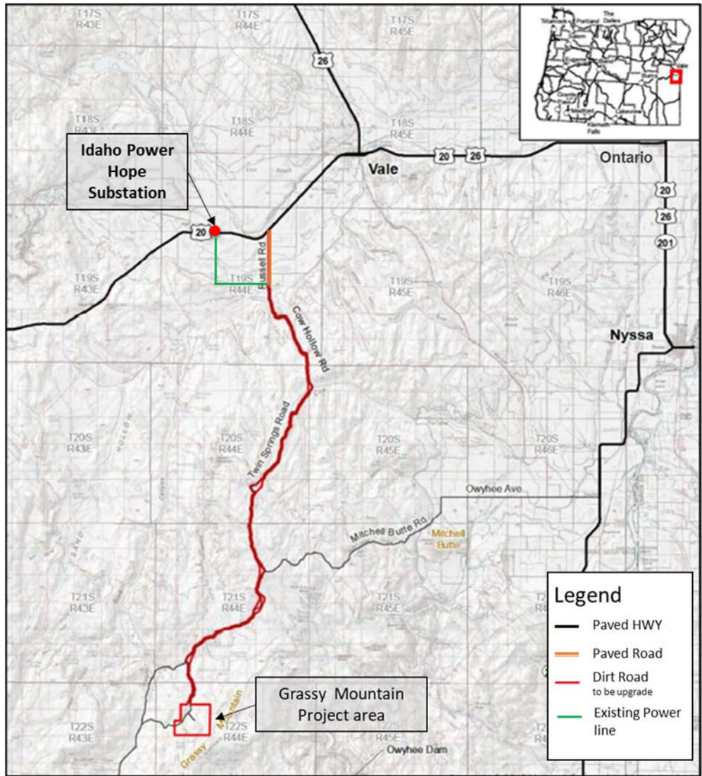
Figure 5-4: Proposed Power Source for the Planned Operation
