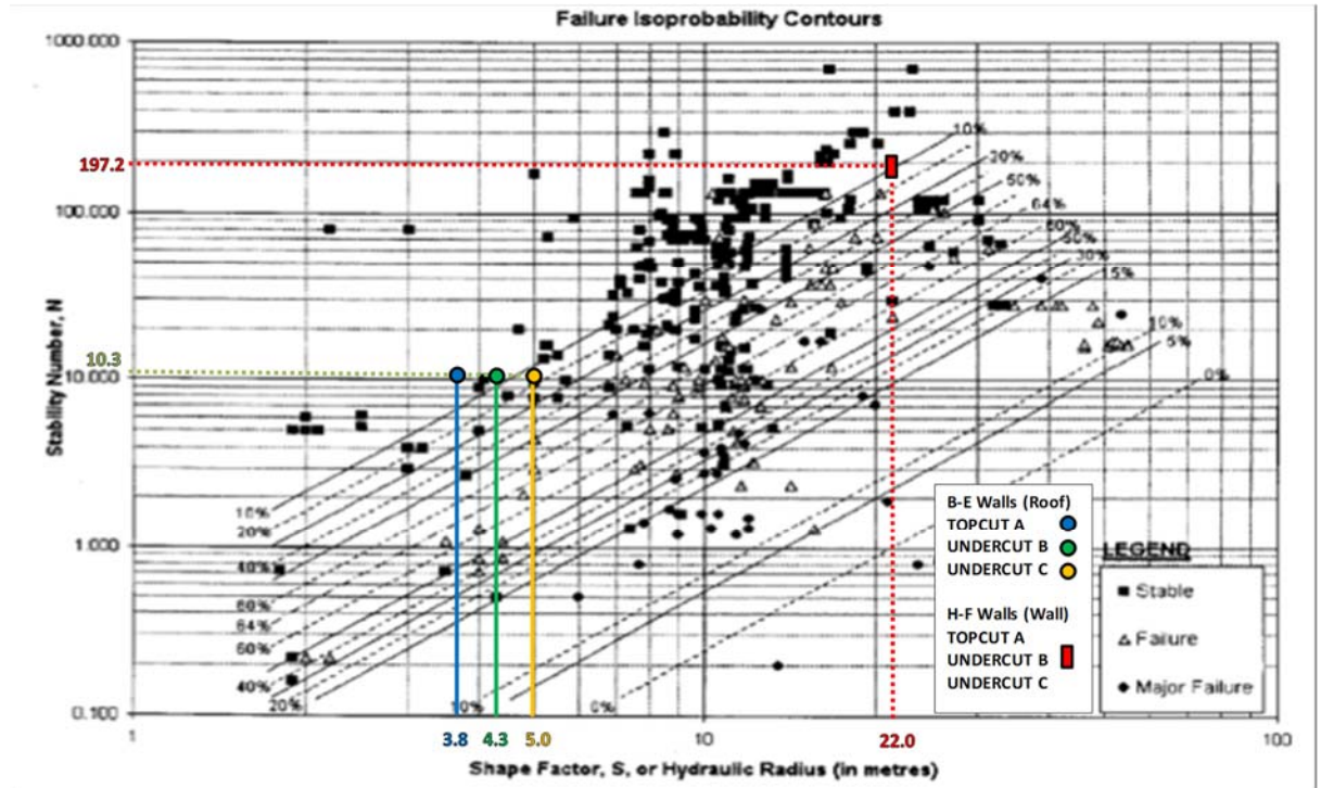
Figure 16-12: Iso-probability contours for failure cases (Mawdesley, 2001).
