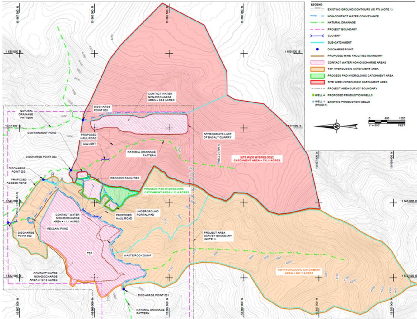
Figure 18-3: Hydrologic Catchment Areas
