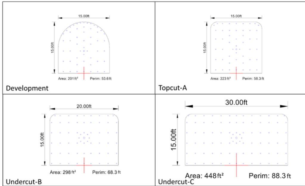
Figure 16-3: Drift Profiles
