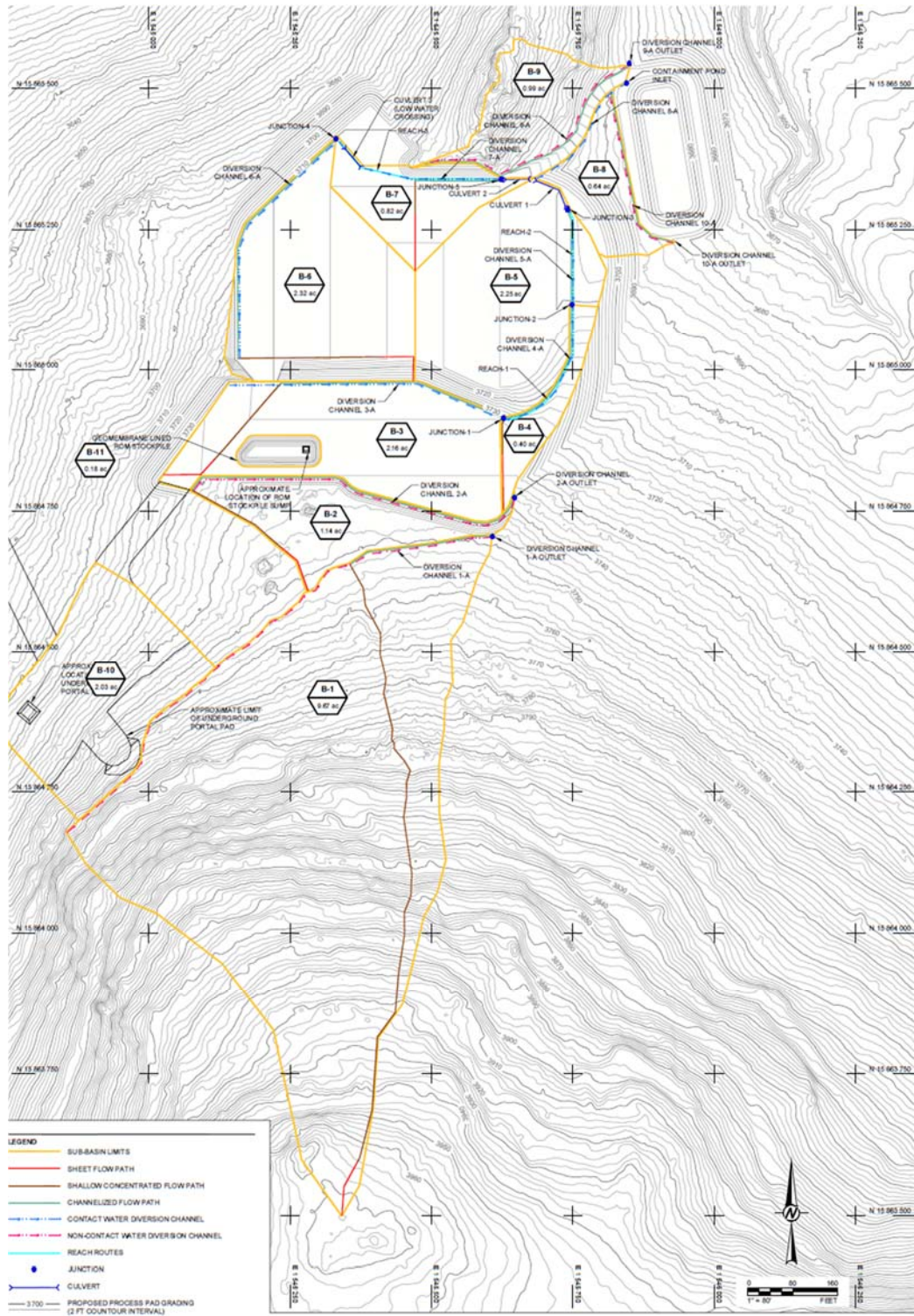
Figure 18-4: Process Plant Stormwater Contact and Non-contact Catchment Areas
