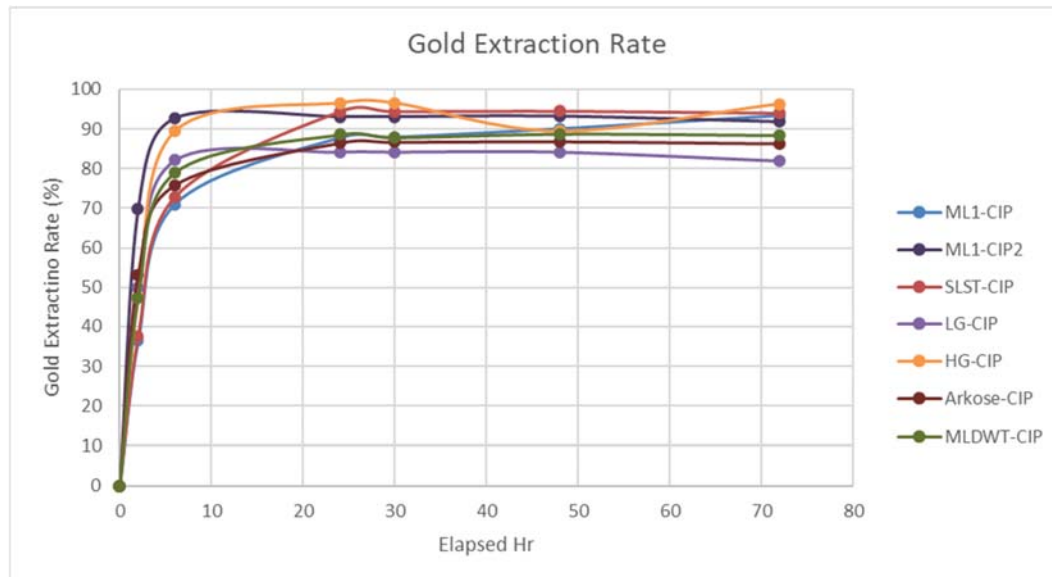
Figure 13-1: Gold Leach Extraction Rate
