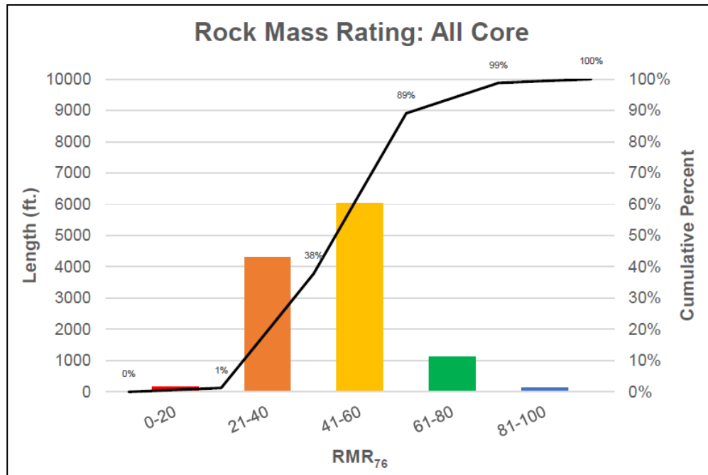
Figure 16-7: Golder Rock Mass Rating (all 2016–2017 core)
