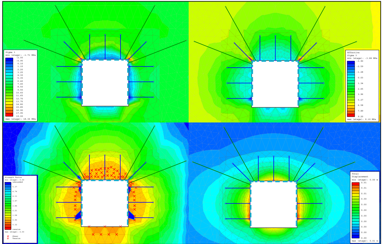
Figure 16-14: Modeling Results for Topcut A; a) Major Principal Stress, S1; b) Minor Principal Stress, S3; c) Strength Factor, SF; d) Displacements, D.
