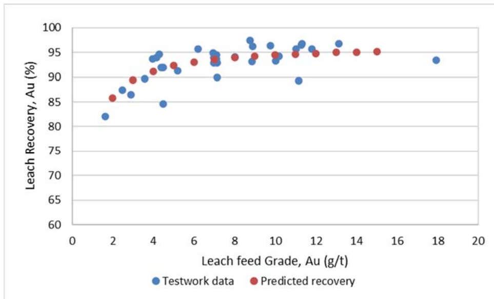
Figure 13-6: Predicted versus Measured Recovery for Gold
