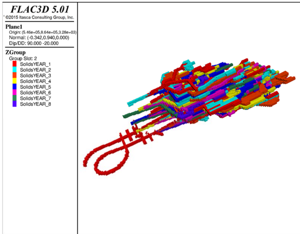
Figure 16-17: Three-Dimensional Model of Finite Difference
