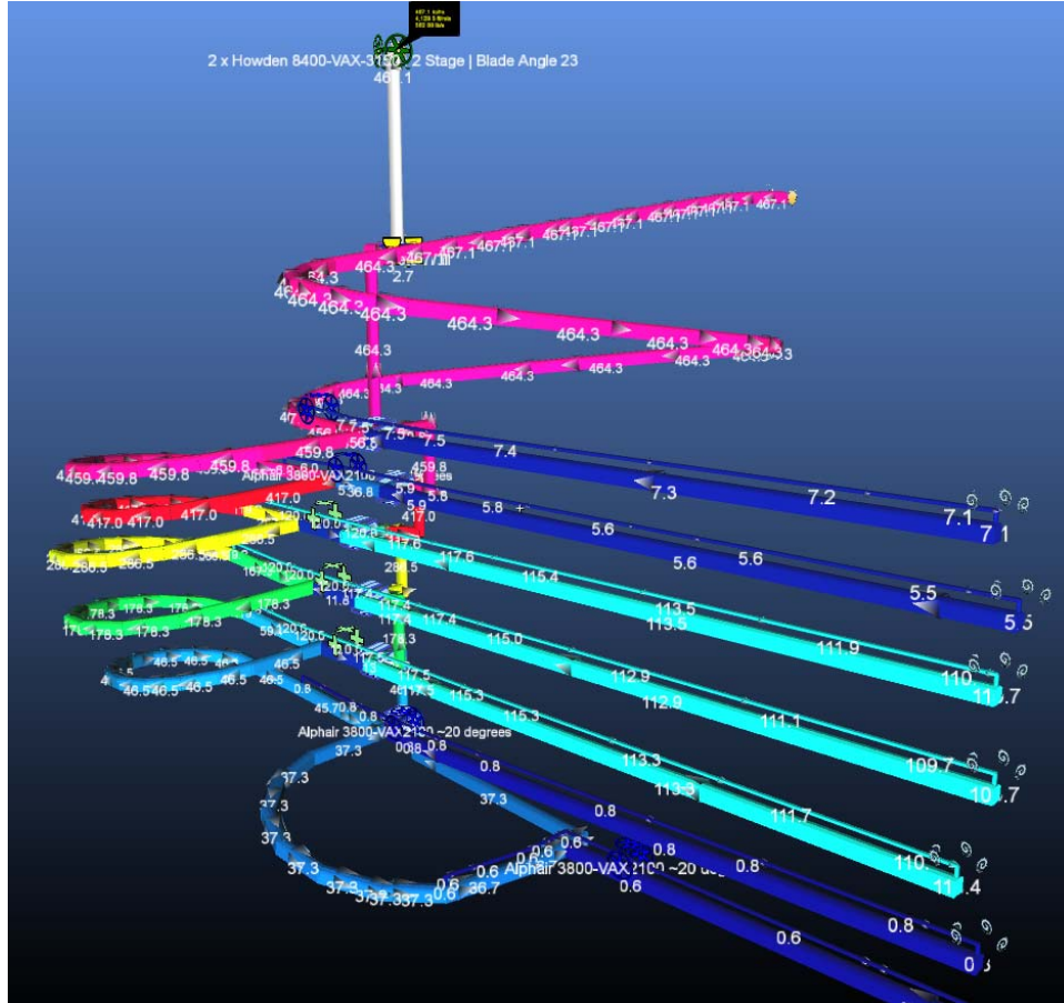
Figure 16-32: Ventilation Network (isometric view looking west)
