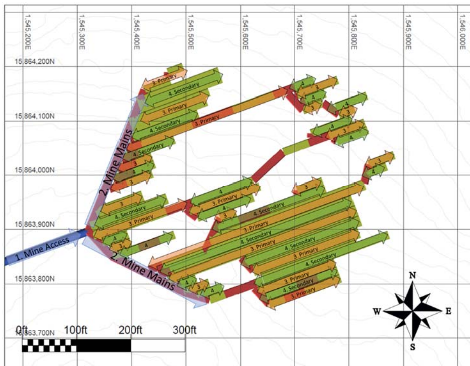
Figure 16-5: Detailed level Sequence for a Typical Level
