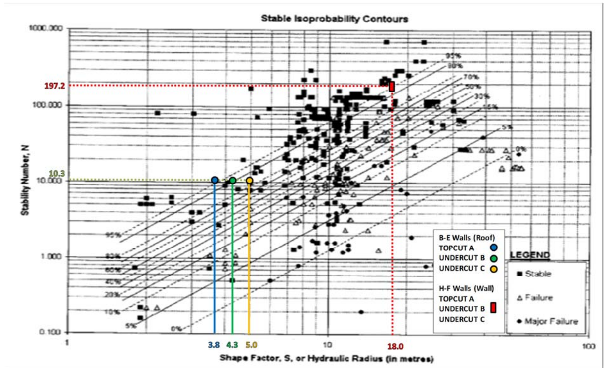
Figure 16-11: Iso-Probability Contours for Stable Cases (Mawdesley, 2001).
