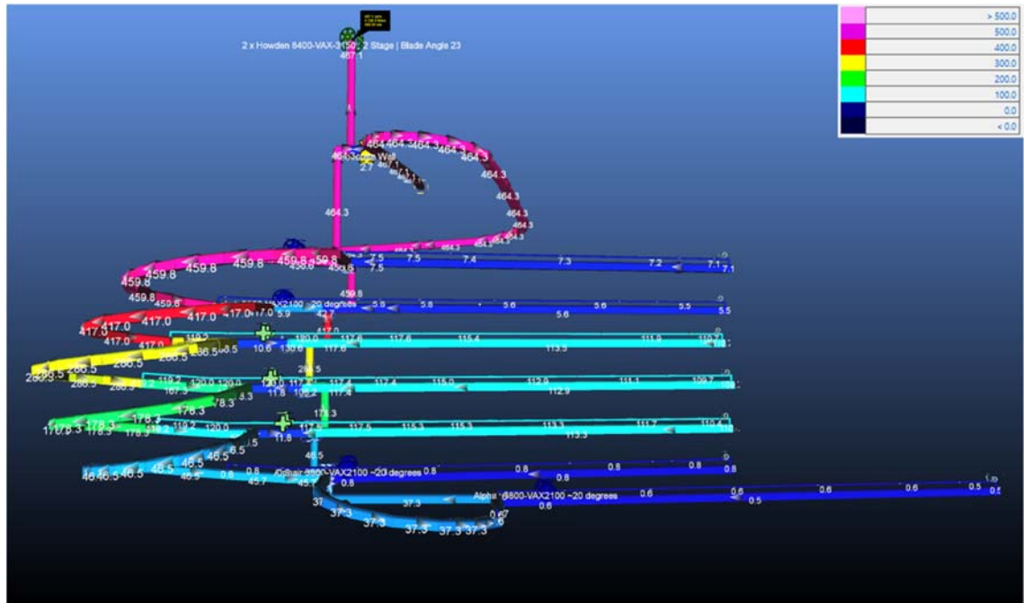
Figure 16-33: Ventilation Network (Section View Looking Northwest)
