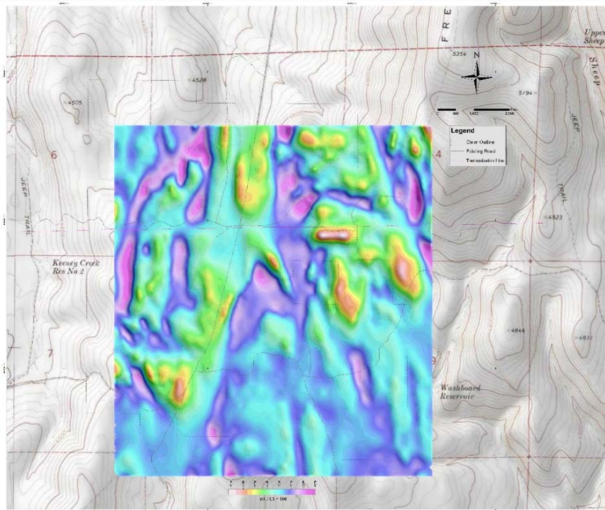
Figure 9-2: 2018 Aerial Magnetic Survey of the Frost Target
