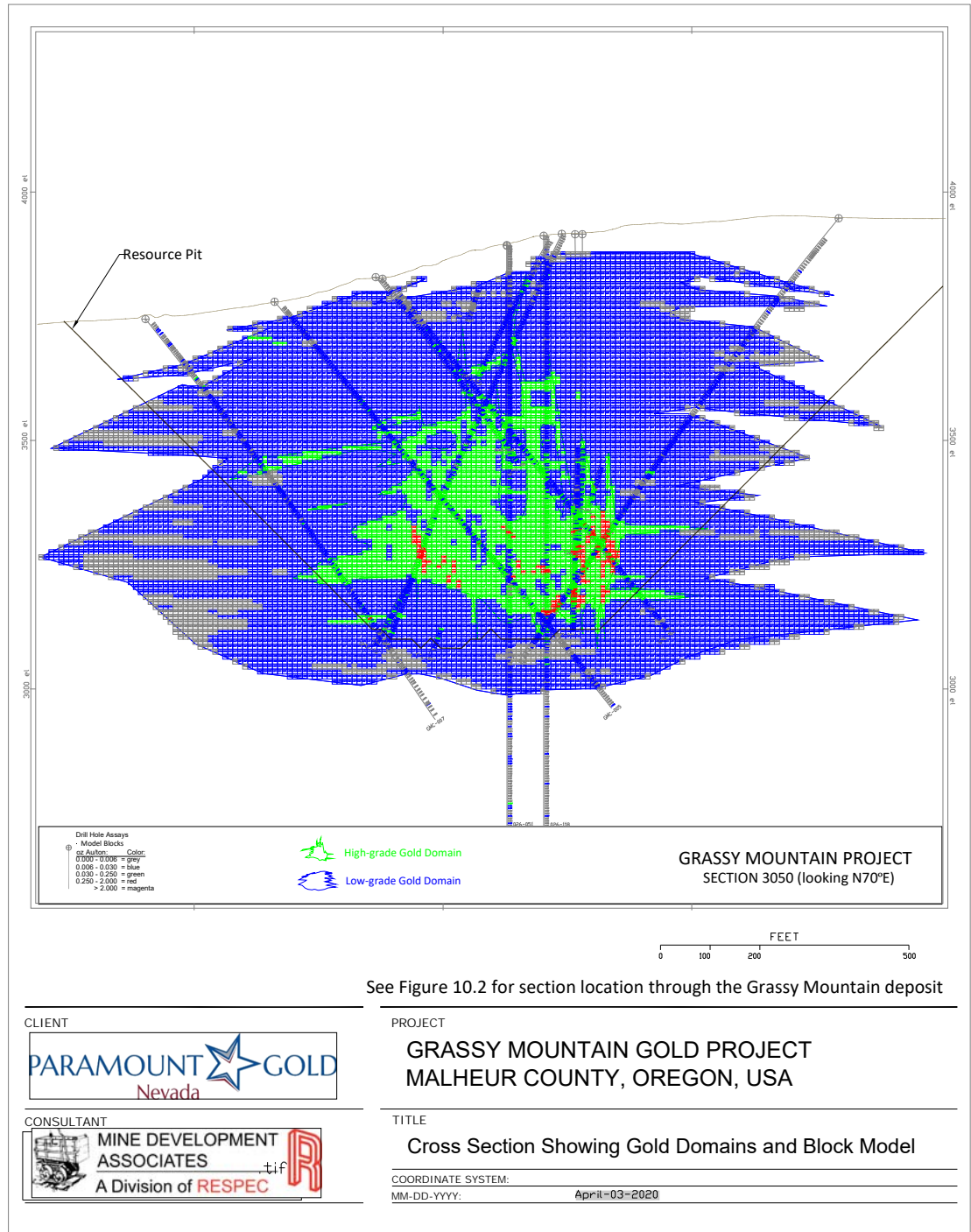
Figure 14-5: Cross Section 3050 Showing Block-Model Gold Grades
