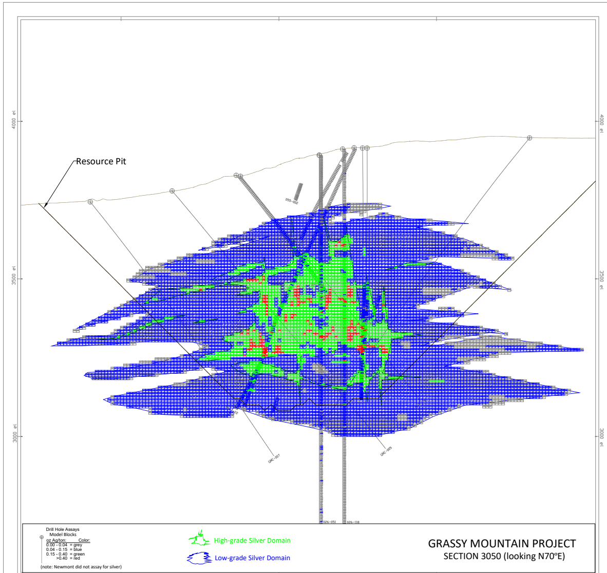
Figure 14-6: Cross Section 3050 Showing Block-Model Silver Grades
