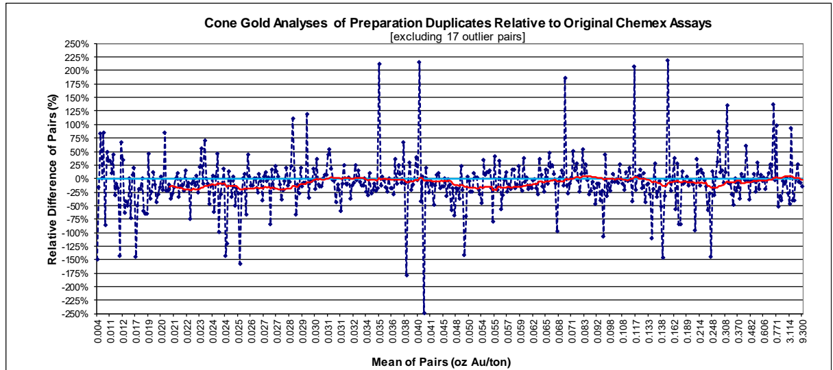
Figure 11-1: Cone Analyses of Preparation Duplicates Relative to Original Chemex Gold Assays
