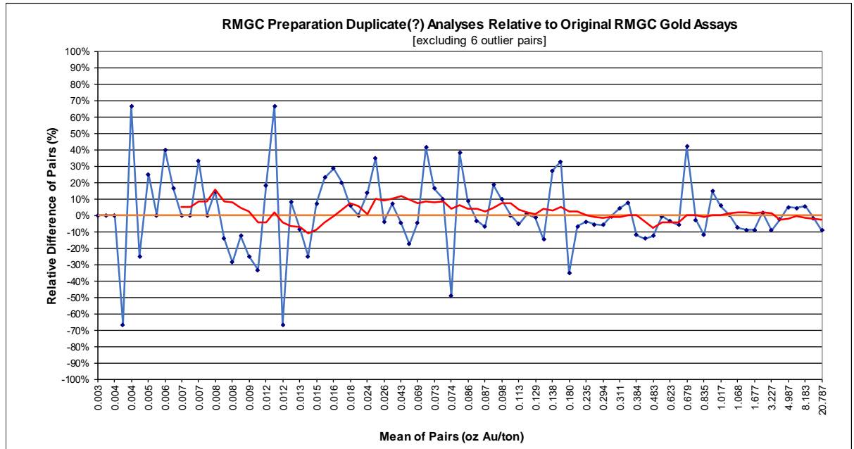
Figure 11-5: RMGC Check Analyses Relative to Original RMGC Gold Assays
