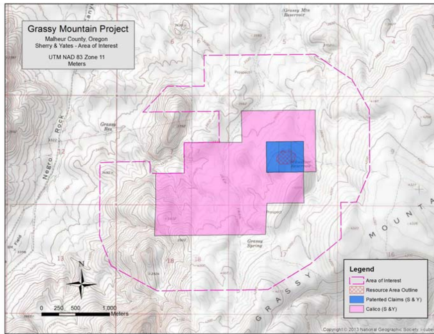
Figure 4-4: Sherry and Yates Area of Interest
