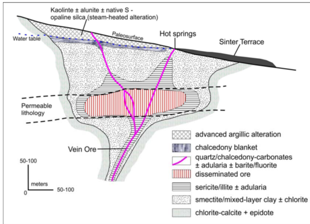
Figure 8-1: Conceptual Hot-Springs Epithermal Deposit Model
