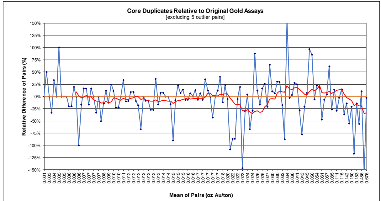
Figure 11-13: Core Duplicates Relative to Original Gold Assays - Paramount
