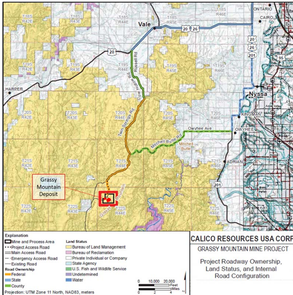
Figure 5-1: Access to Grassy Mountain Claims Group
