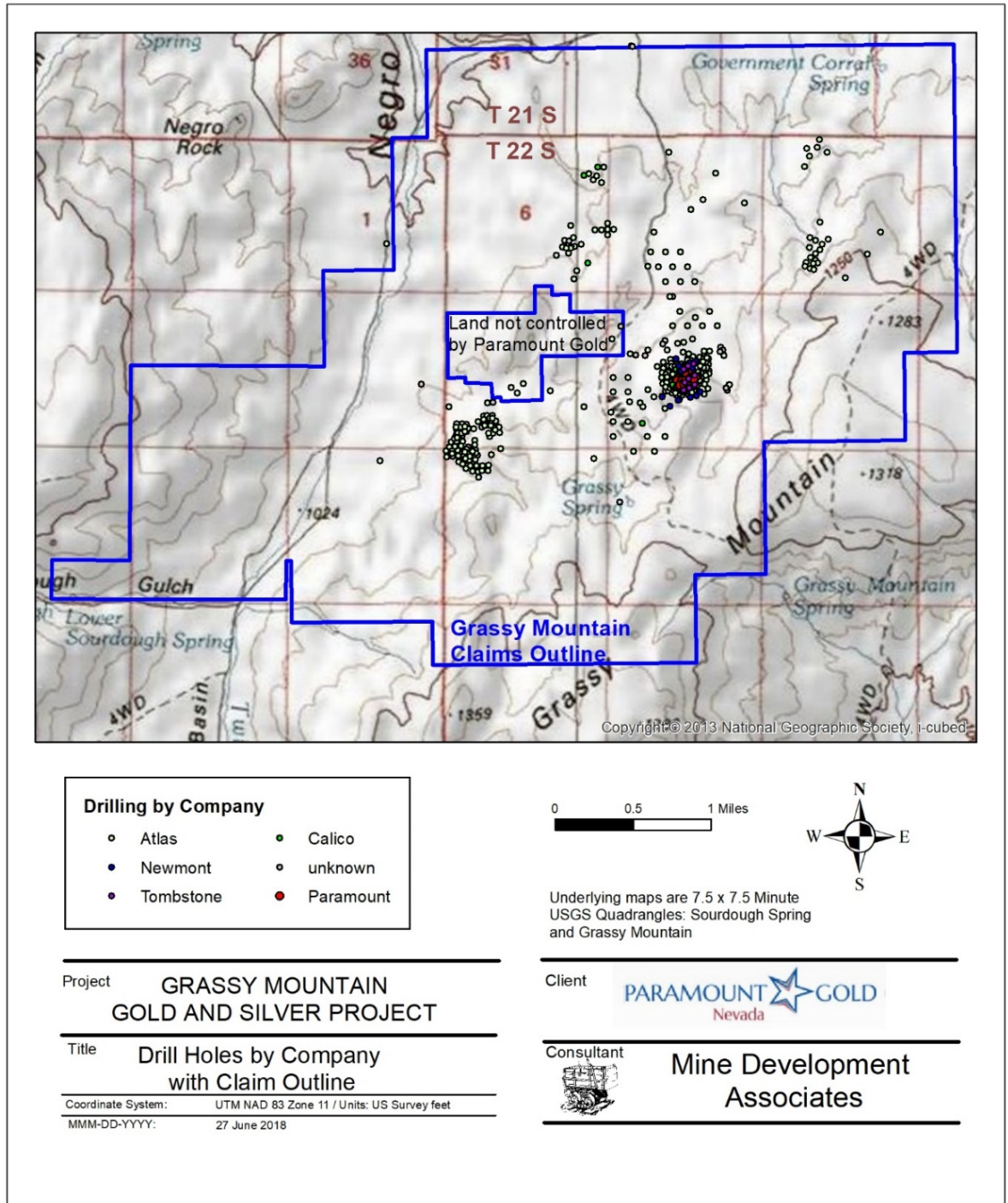
Figure 10-1: Locations of All Drill Holes Within the Grassy Mountain Claim Block
