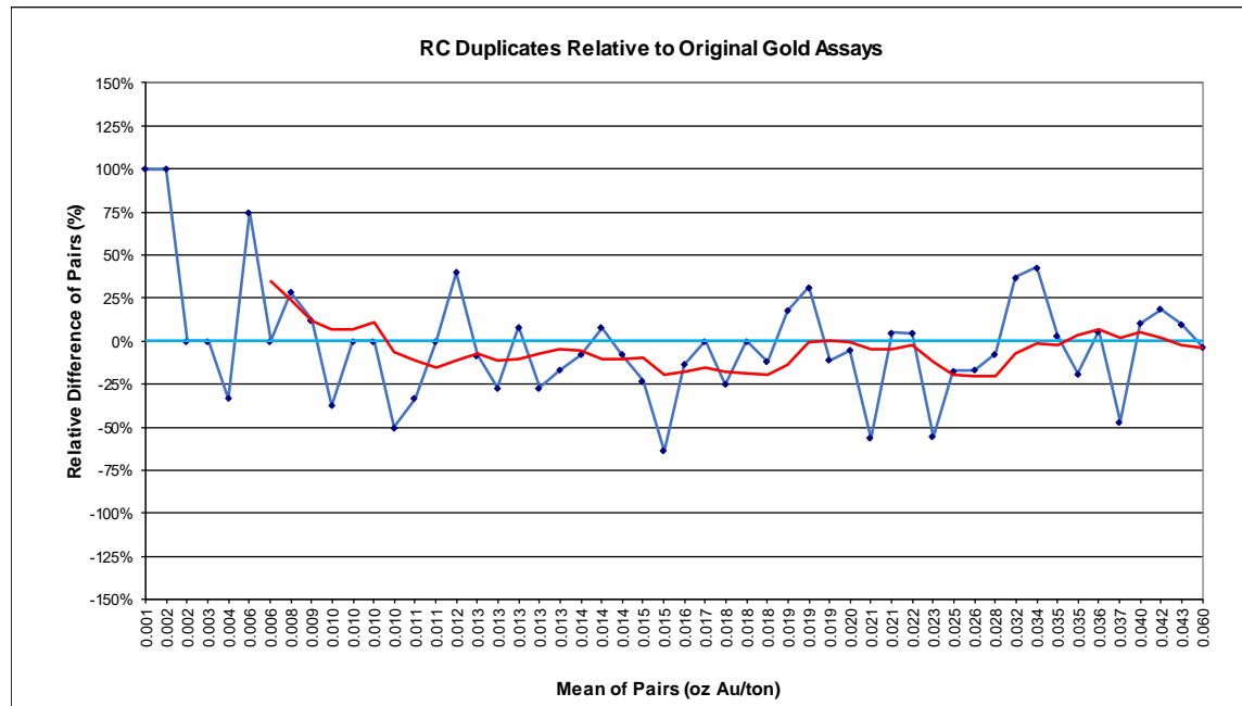
Figure 11-15: Paramount RC Duplicates Relative to Original Gold Analyses
