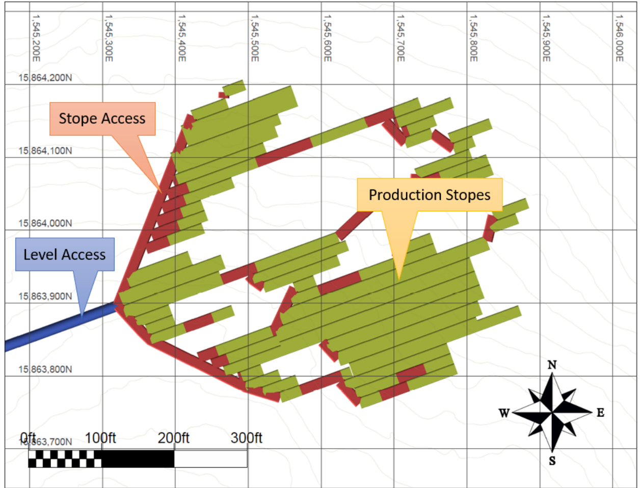
Figure 15-1: Mine Production Design of Level 3210, Plan View
