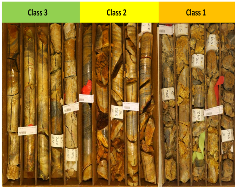
Figure 16-9: Examples of Three Geotechnical Rock Classes
