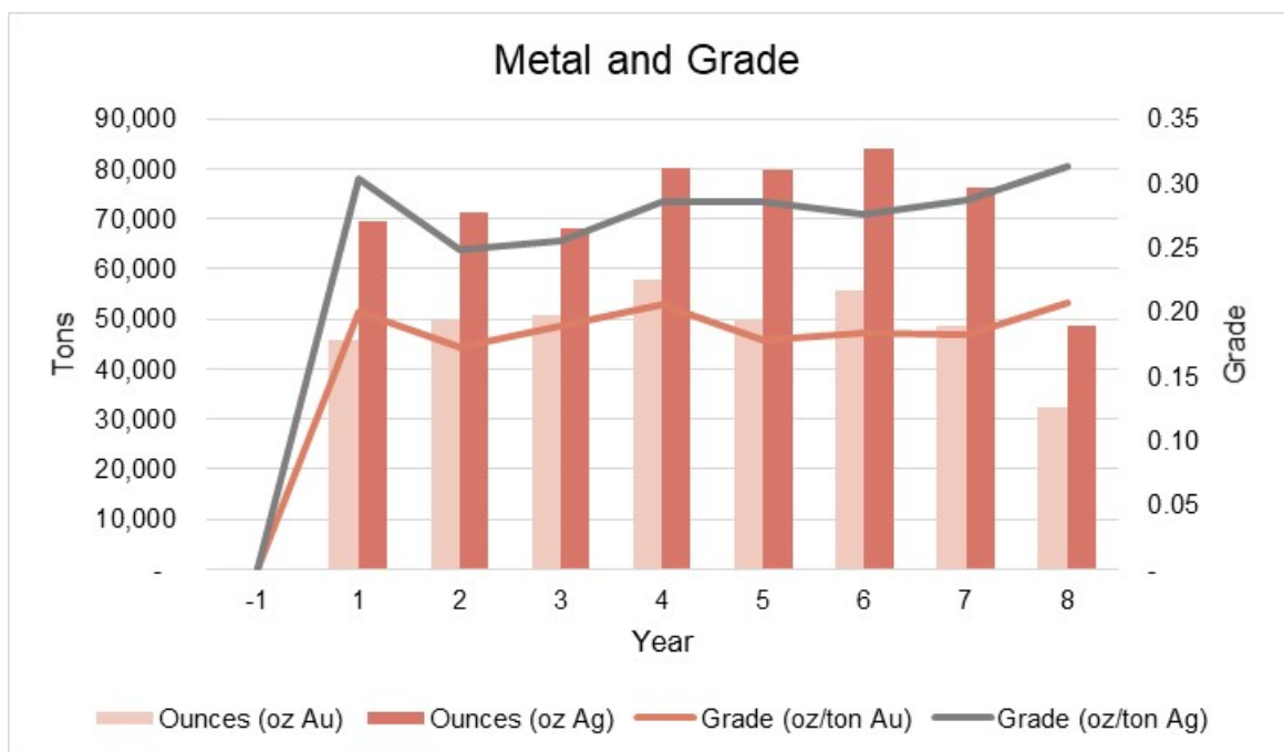
Figure 16-38: Mine Production Schedule (ounces by period)
