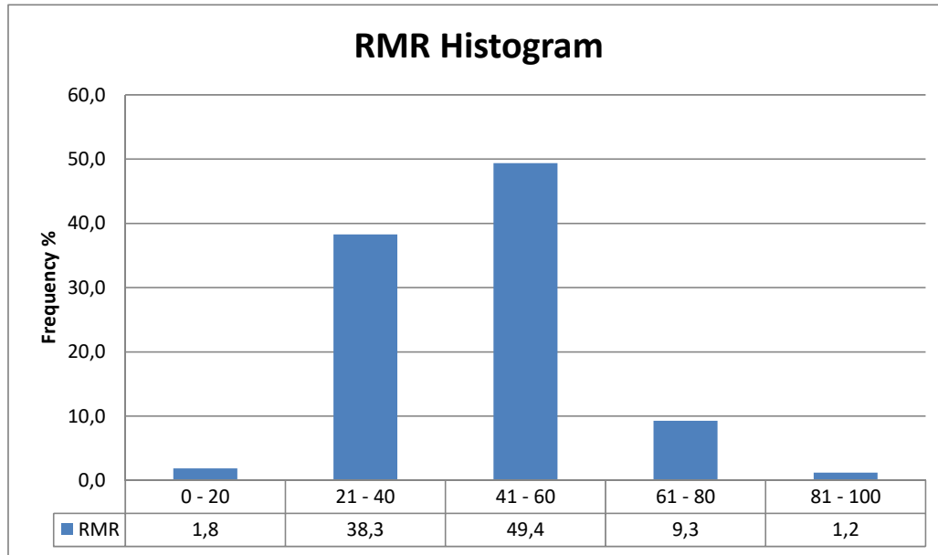
Figure 16-8: RMR 76 Histogram from 27 Drill Holes.
