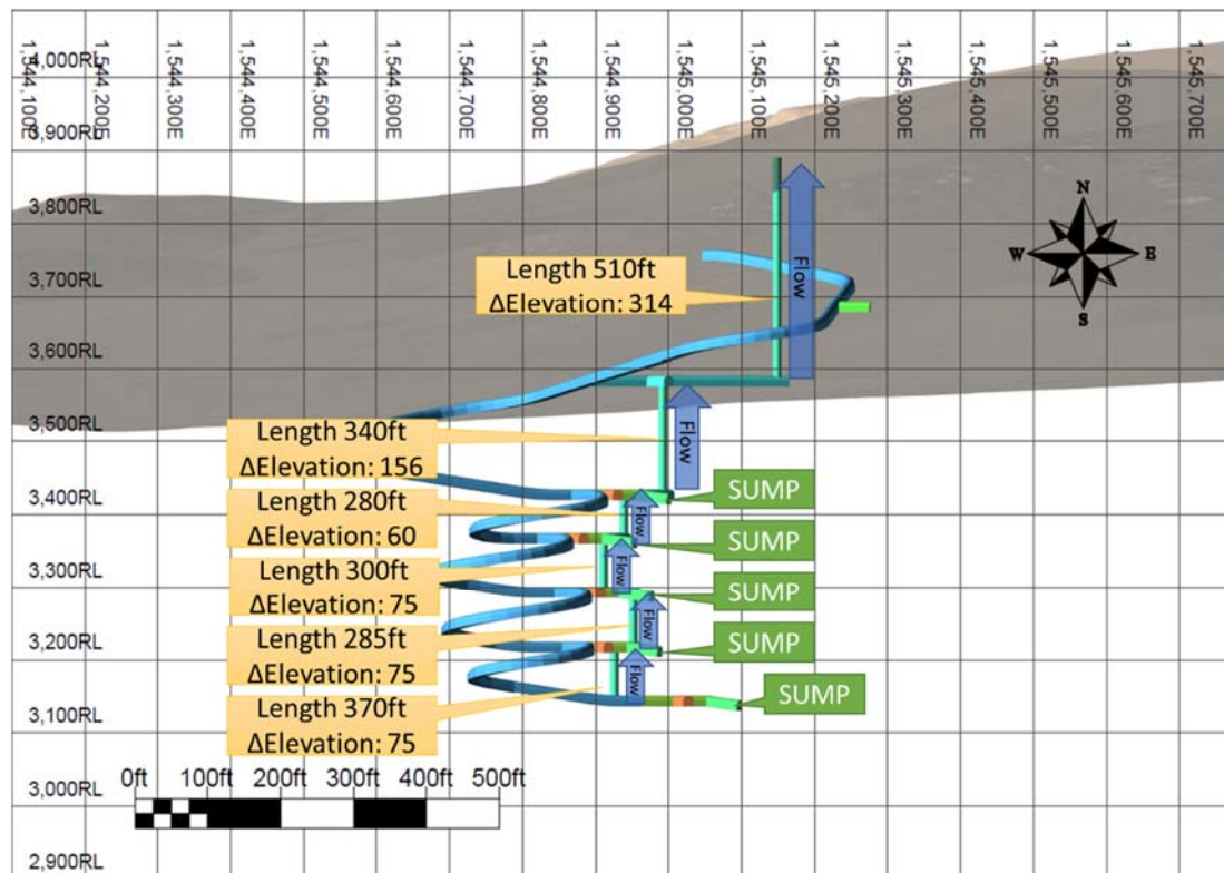
Figure 16-35: Sump Design and Layout
