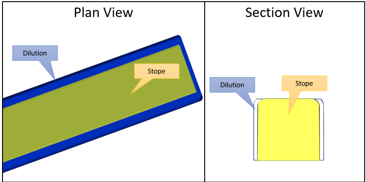
Figure 15-2: External Dilution Scheme at Level 3240
