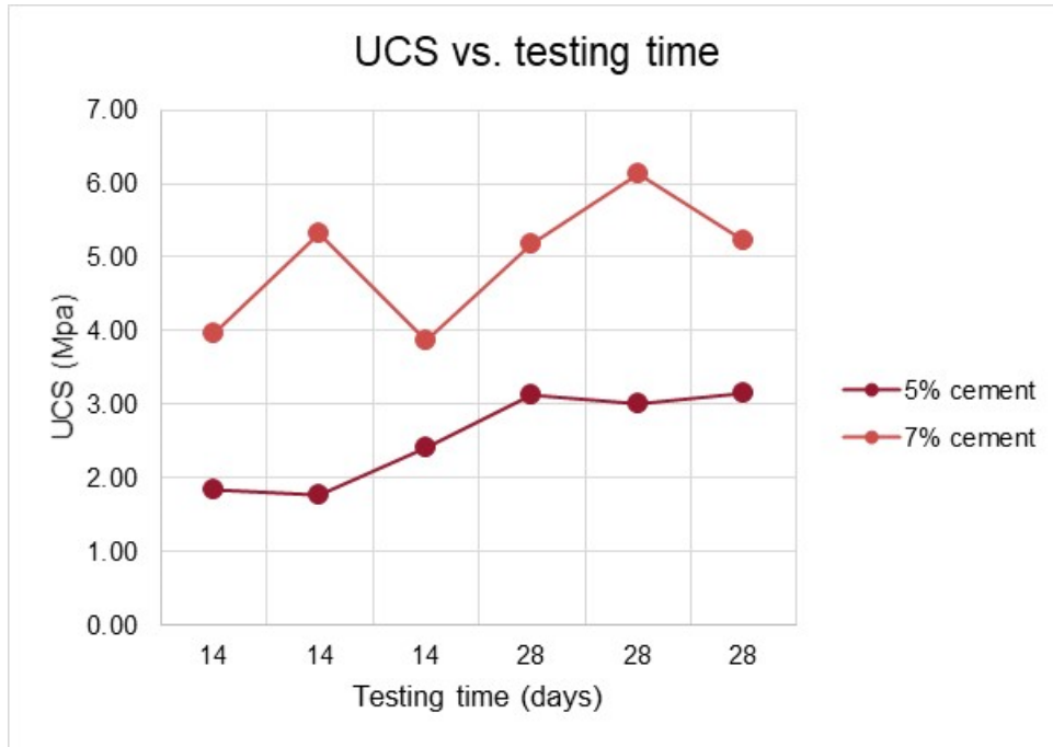
Figure 16-30: UCS Results vs Curing Time
