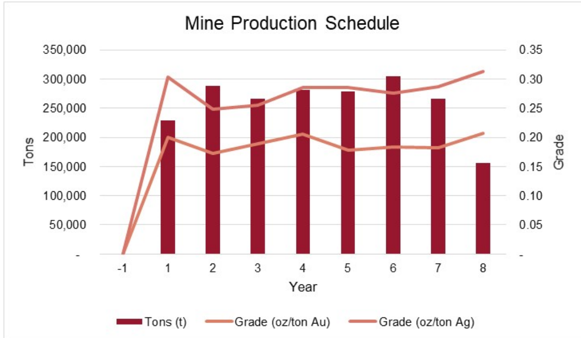
Figure 16-37: Mine Production Schedule (tons by period)
