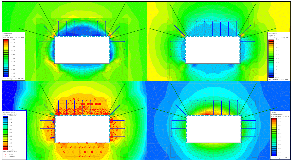
Figure 16-16: Modeling Results for Undercut C; a) Major Principal Stress, S1; b) Minor Principal Stress, S3; c) Strength Factor, SF; d) Displacements, D.
