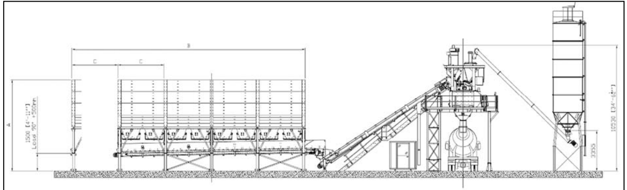
Figure 16-31: Eagle 4000 Backfill Plant
