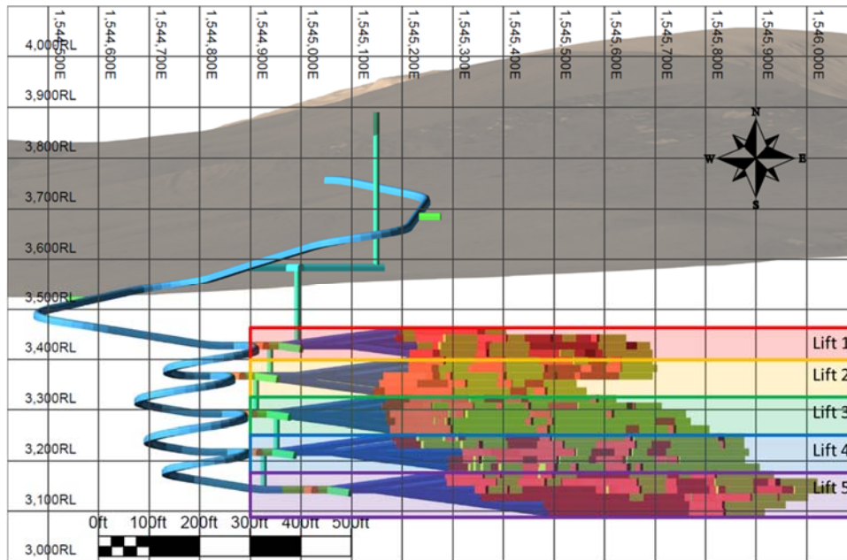
Figure 16-6: Mining Lifts
