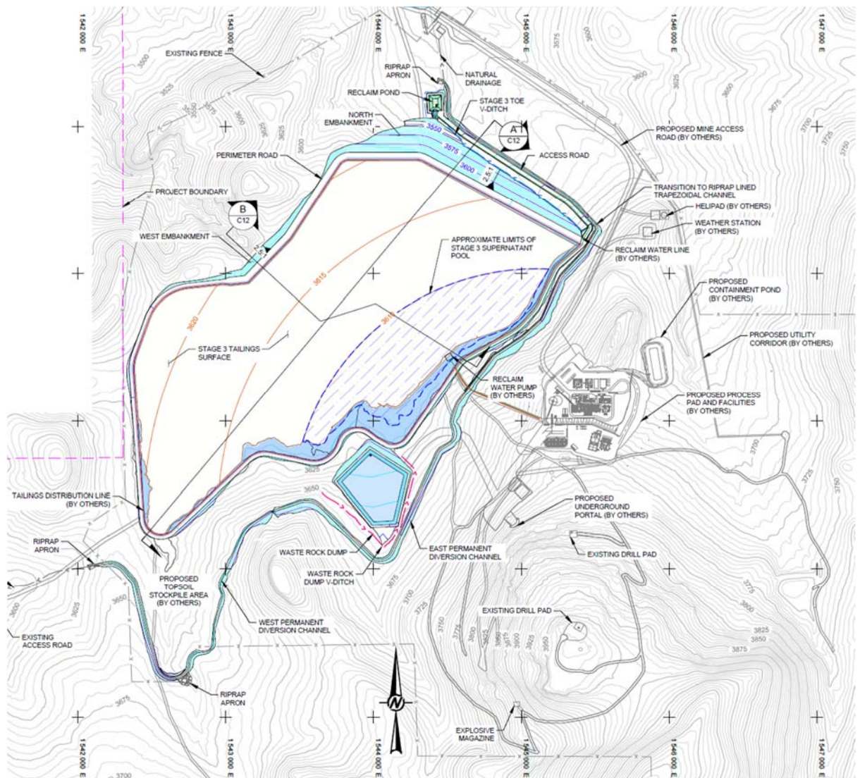
Figure 18-2: Proposed TSF
