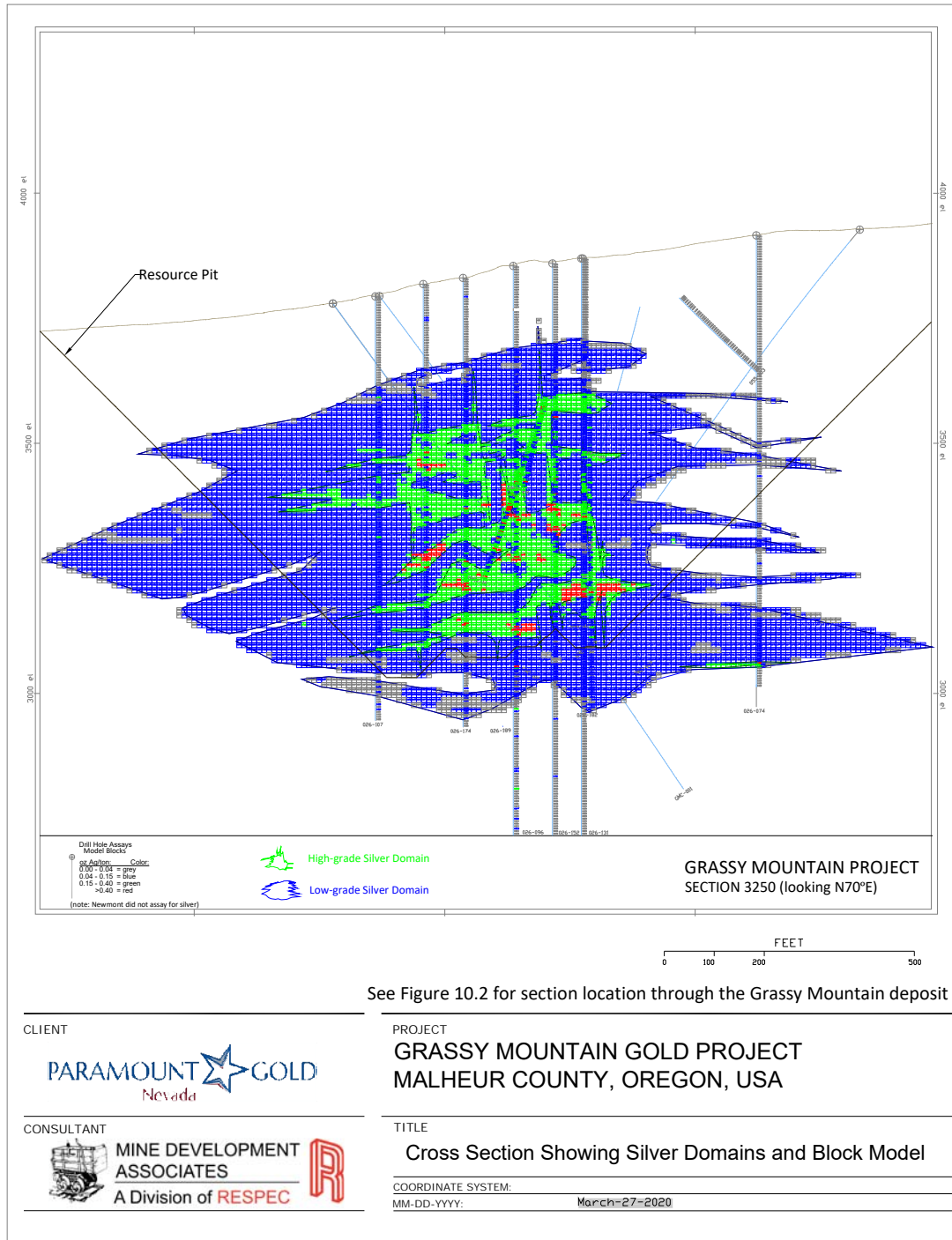
Figure 14-8: Cross Section 3250 Showing Block-Model Silver Grades
