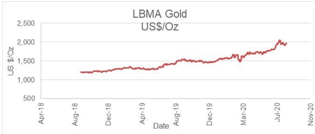
Figure 19-1: London Bullion Market Association Gold Price (2-year span, US$/oz)
