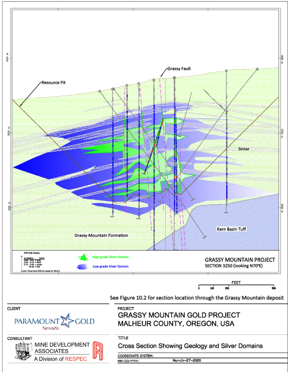
Figure 14-4: Cross Section 3250 Showing Silver Domains
