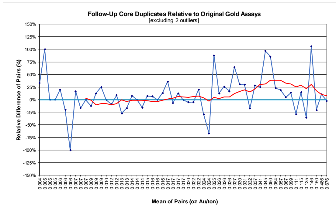
Figure 11-14: Second Set of Paramount Core Duplicates Relative to Original Gold Assays
