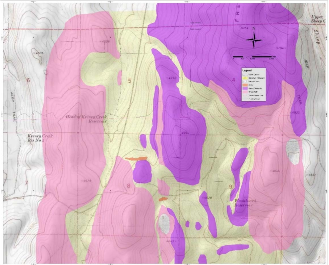
Figure 7-4: Frost Claims Group Geologic Map
