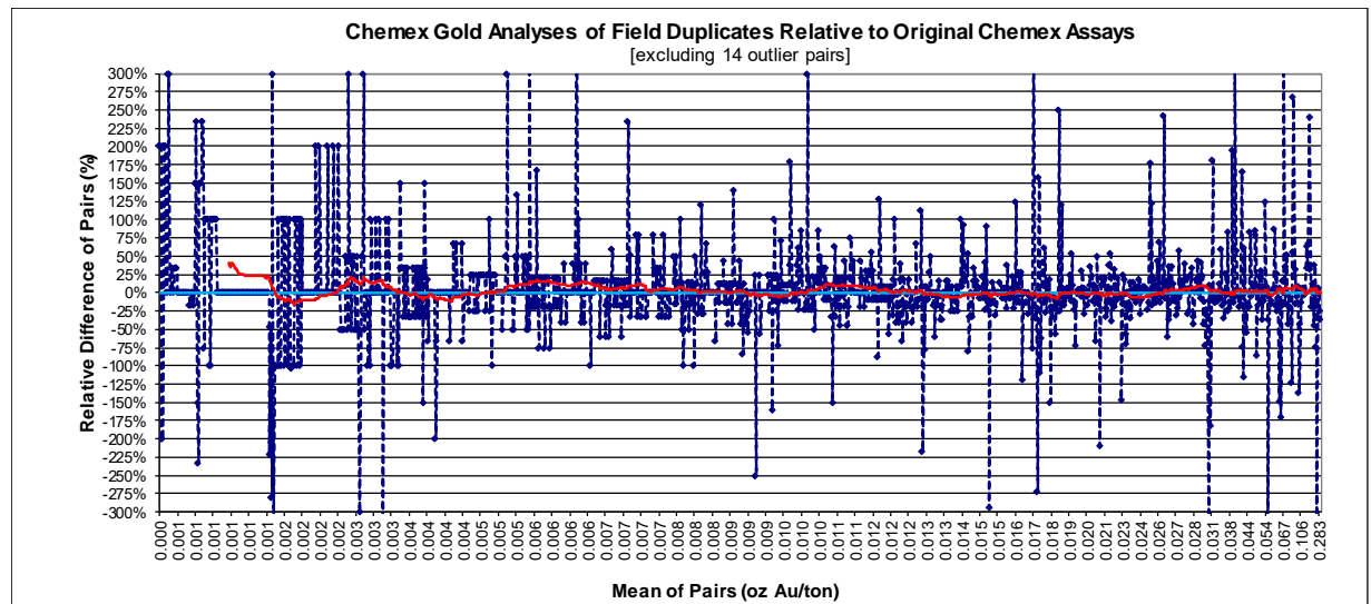
Figure 11-3: Chemex Analyses of RC Field Duplicates Relative to Original Chemex Gold Assays
