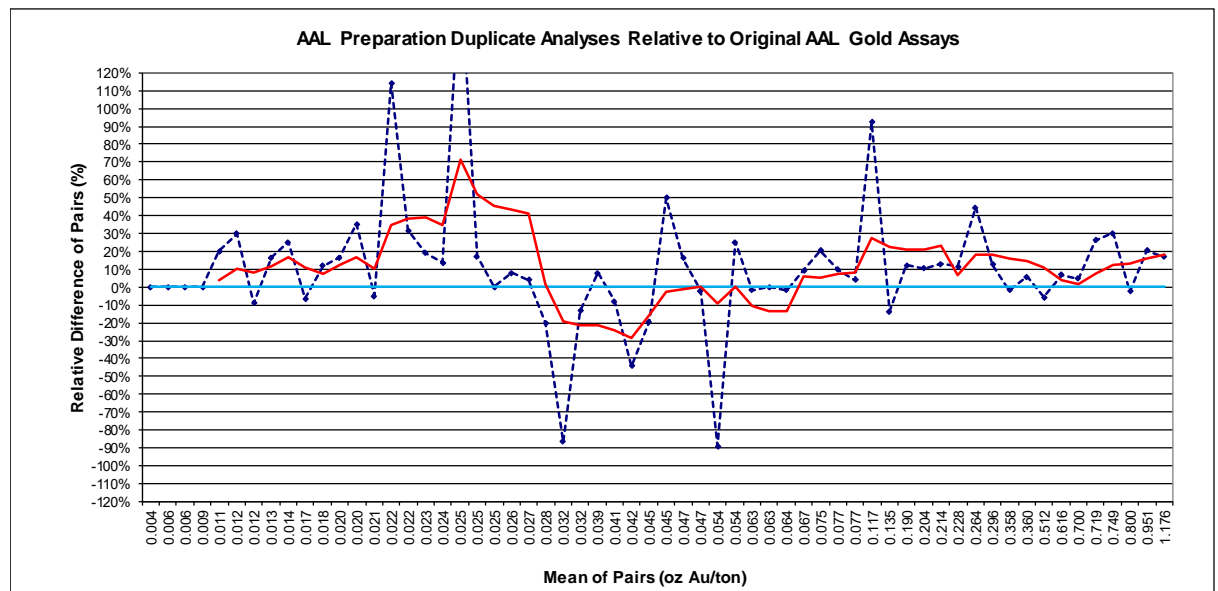
Figure 11-7: AAL Preparation Duplicate Analyses Relative to AAL Original Gold Assays
