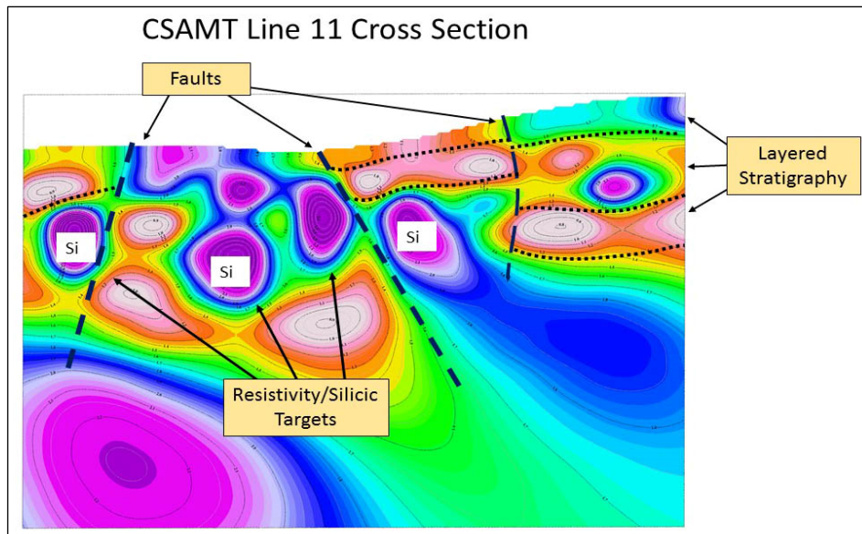
Figure 9-4: Cross Section Generated by 2019 CSAMT Data at Frost Target
