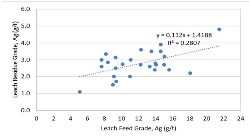
Figure 13-5: Relationship Between Leach Feed and Residue Grades for Silver
