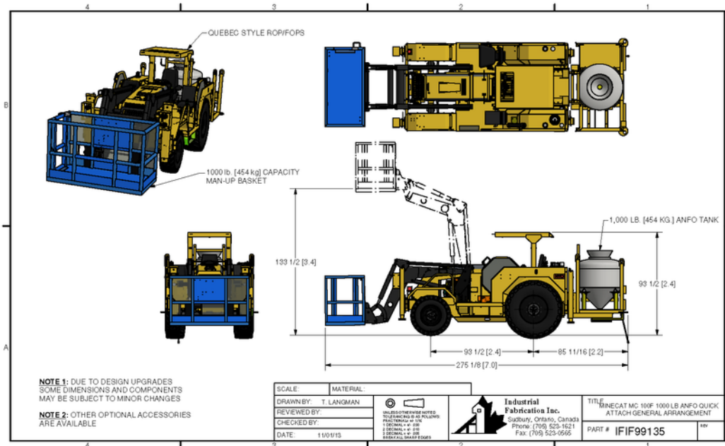
Figure 16-24: CAT 440 with Emulsion Configuration
