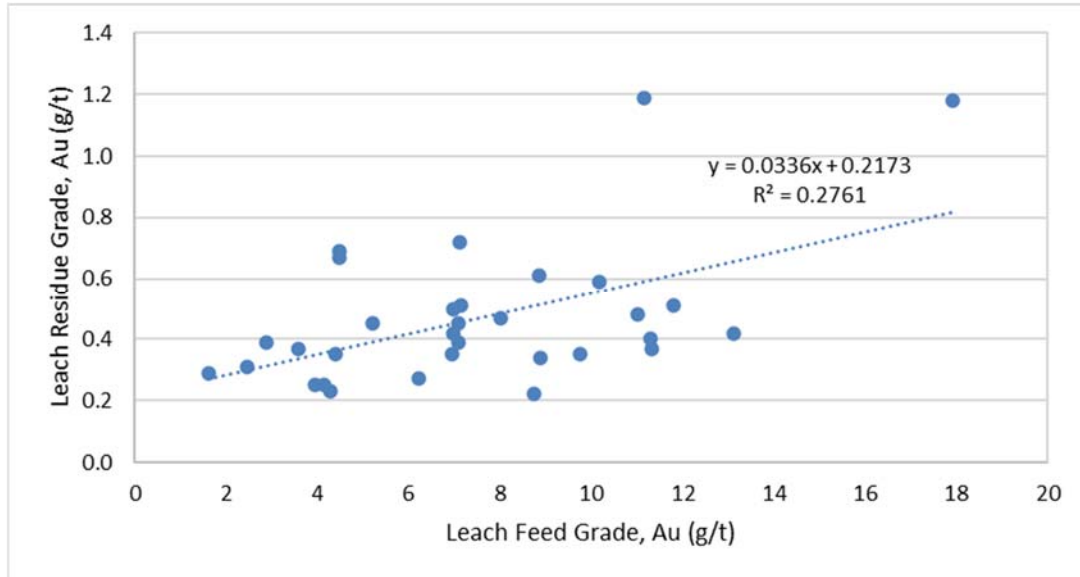
Figure 13-4: Relationship Between Leach Feed and Residue Grades for Gold
