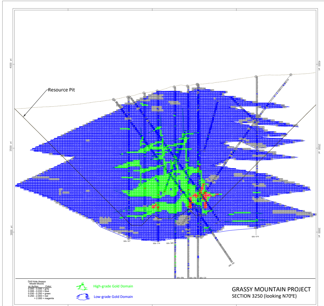
Figure 14-7: Cross Section 3250 Showing Block-Model Gold Grades
