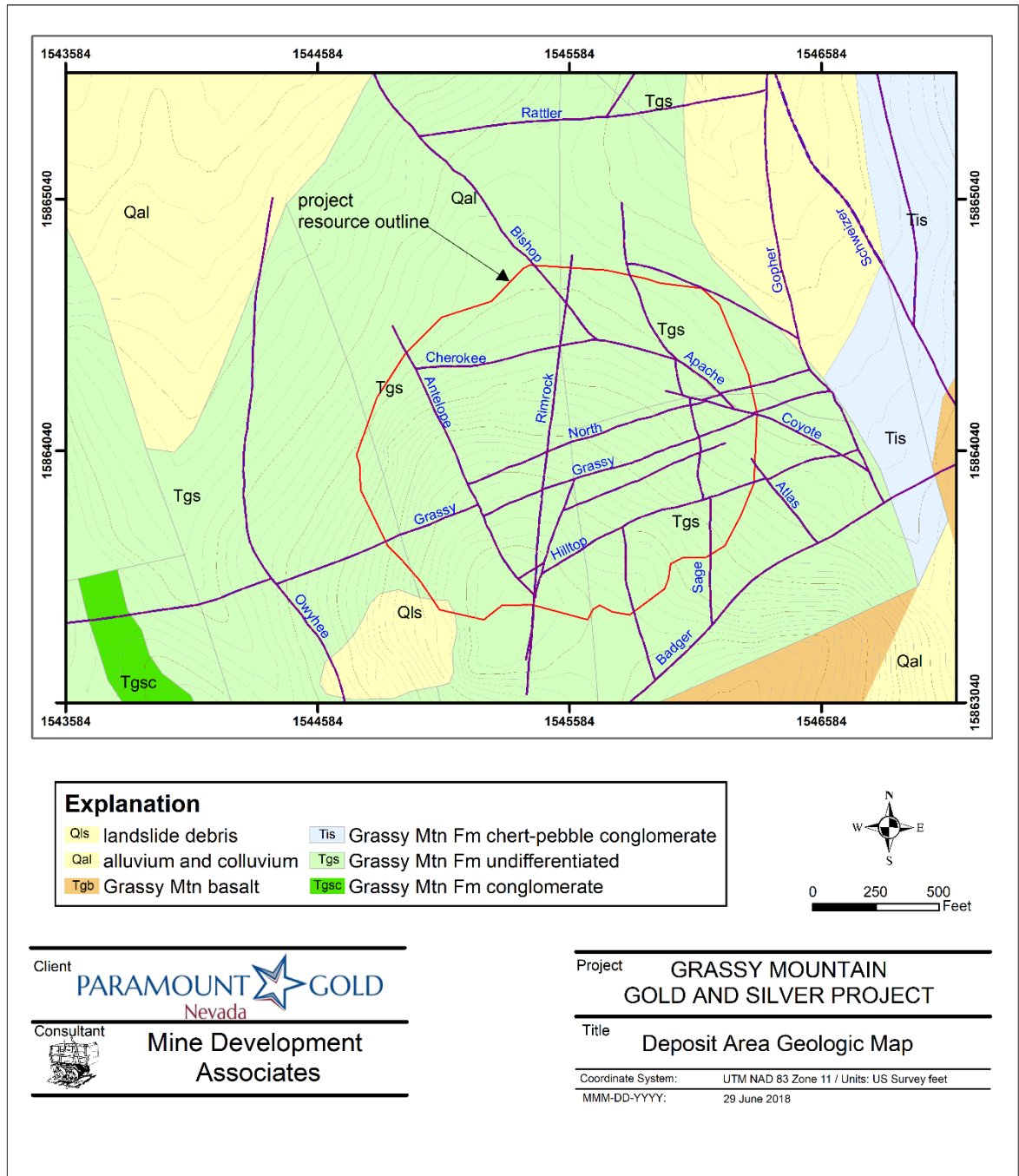
Figure 7-3: Grassy Mountain Deposit Area Geologic Map
