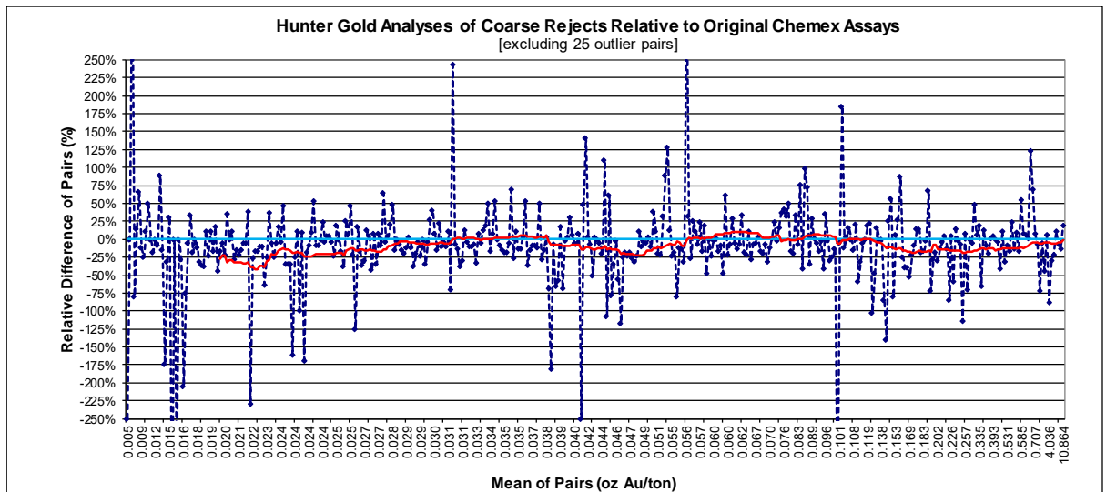
Figure 11-2: Hunter Analyses of Preparation Duplicates Relative to Original Chemex Gold Assays
