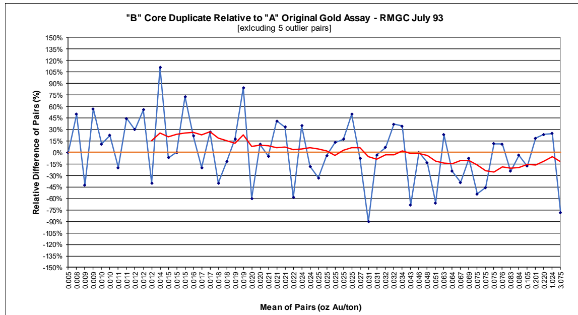
Figure 11-6: RMGC Core Duplicate “B” Relative to RMGC “A” Gold Assays
