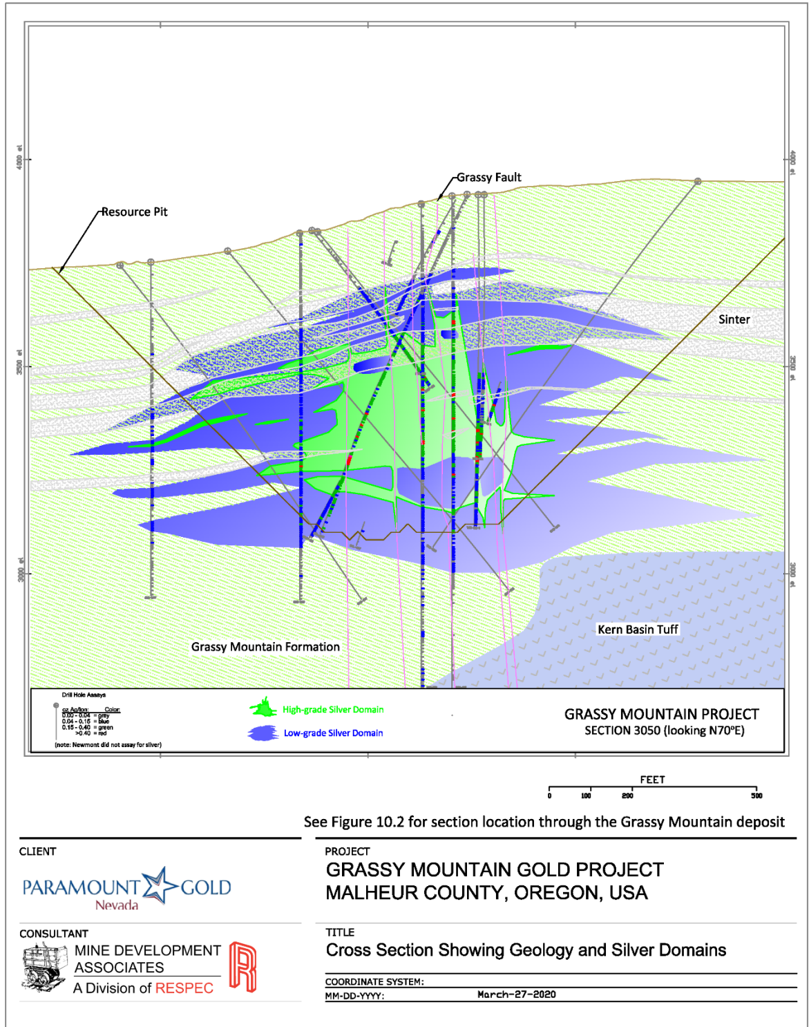
Figure 14-2: Cross Section 3050 Showing Silver Domains
