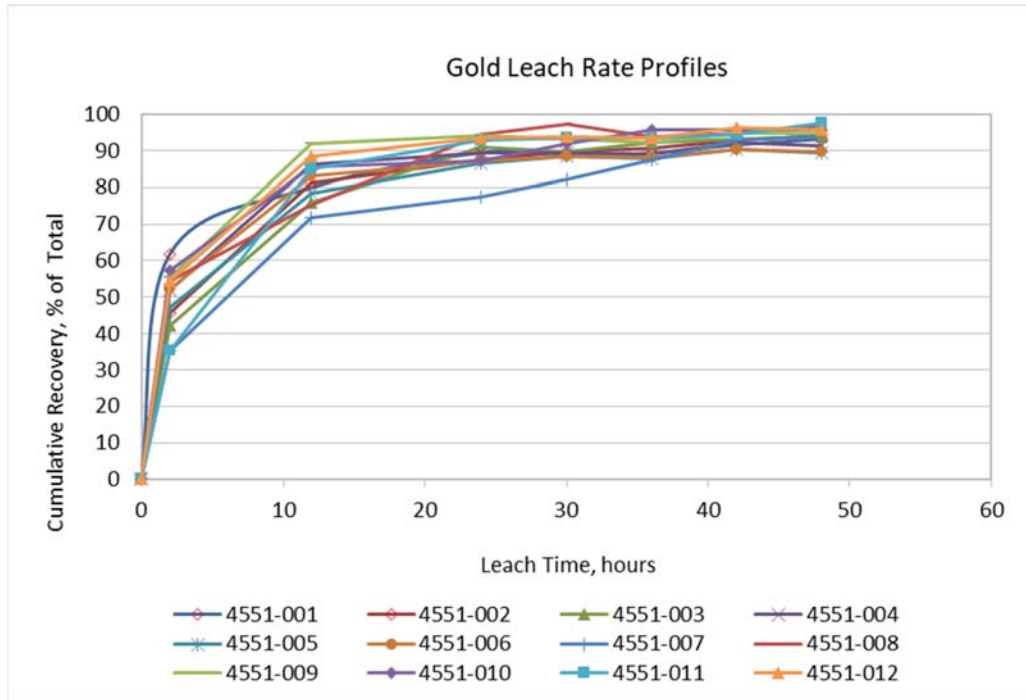
Figure 13-2: Gold Leach Extraction Rate for Grade Variability Samples
