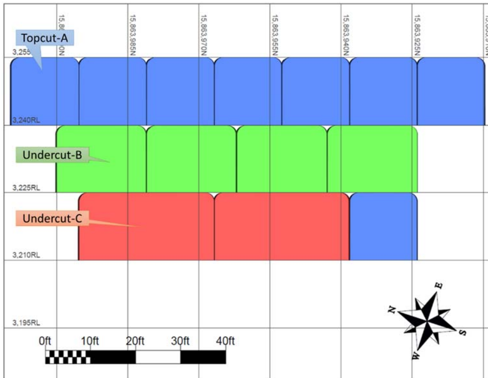
Figure 16-4: Production Drift Layout (Section Looking East)
