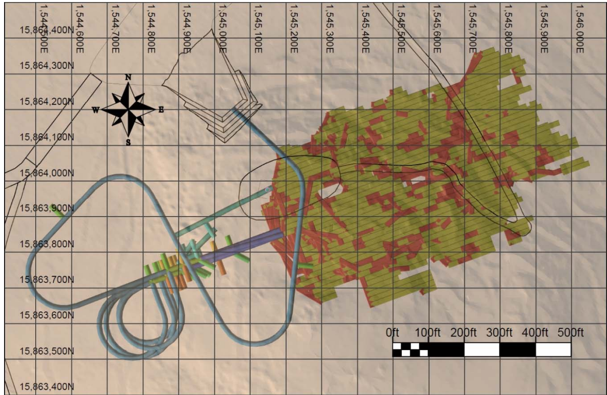
Figure 16-2: Proposed Grassy Mountain Mine Plan (plan view)
