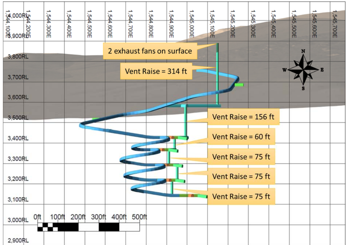
Figure 16-34: Design of Vent Raises
