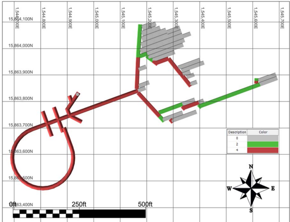
Figure 16-23: 3360 Shotcrete Thickness (units in inches)
