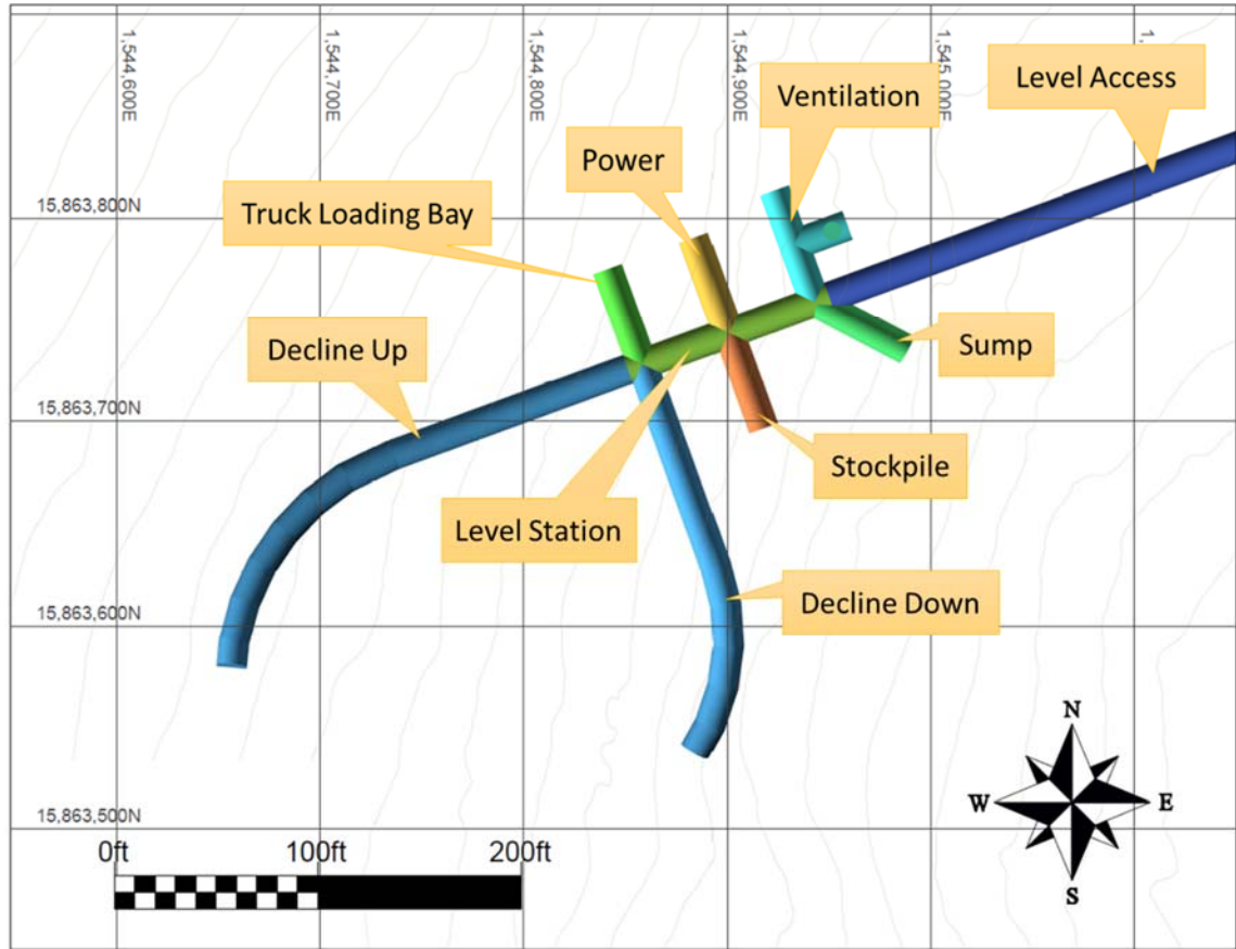
Figure 16-19: Station Design
