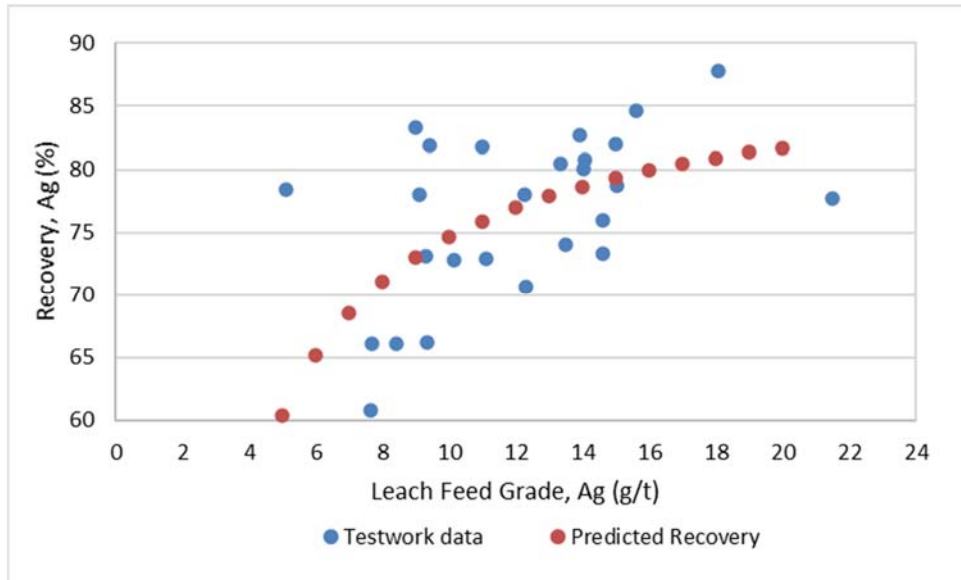
Figure 13-7: Predicted versus Measured Recovery for Silver
