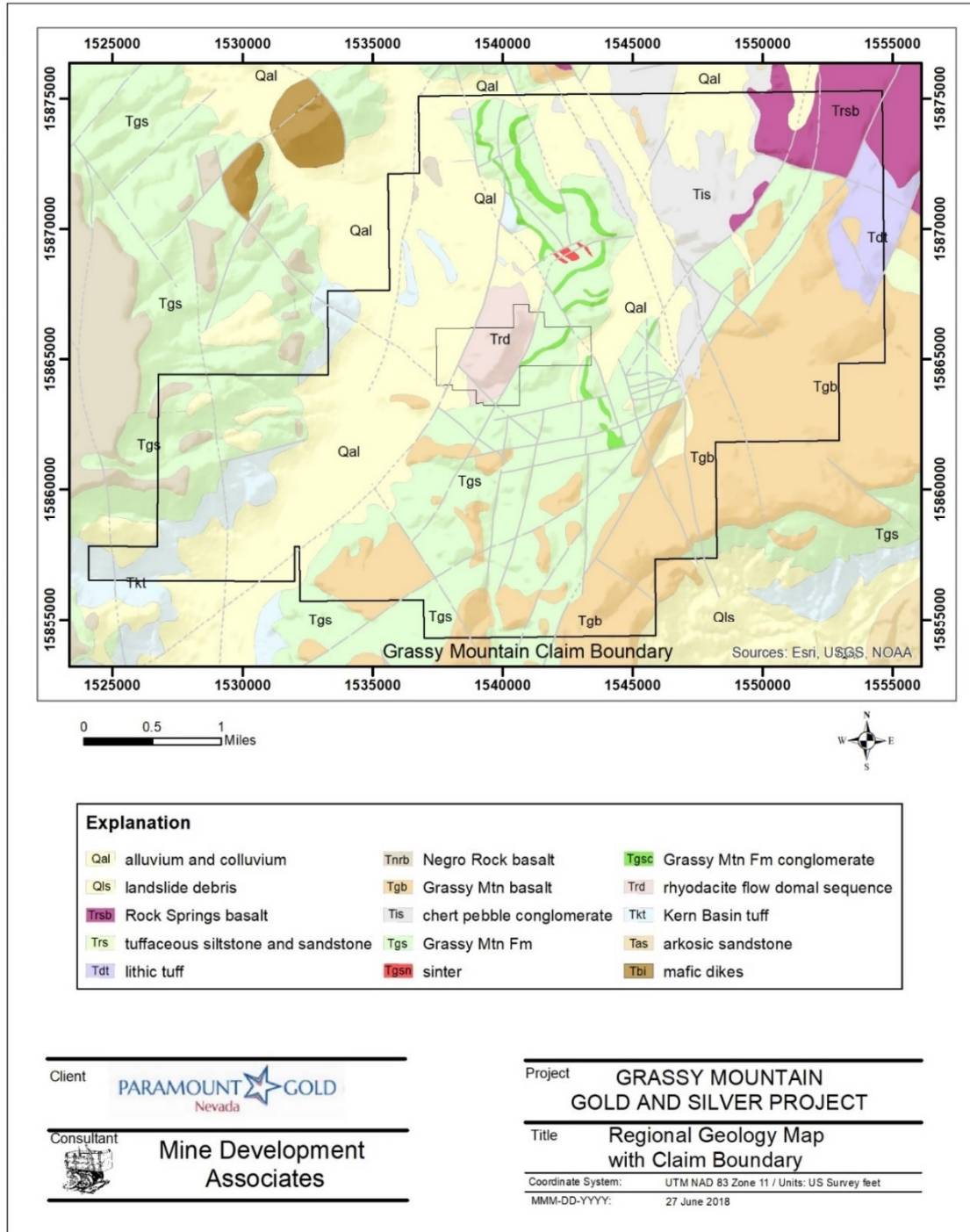
Figure 7-1: Grassy Mountain Regional Geology
