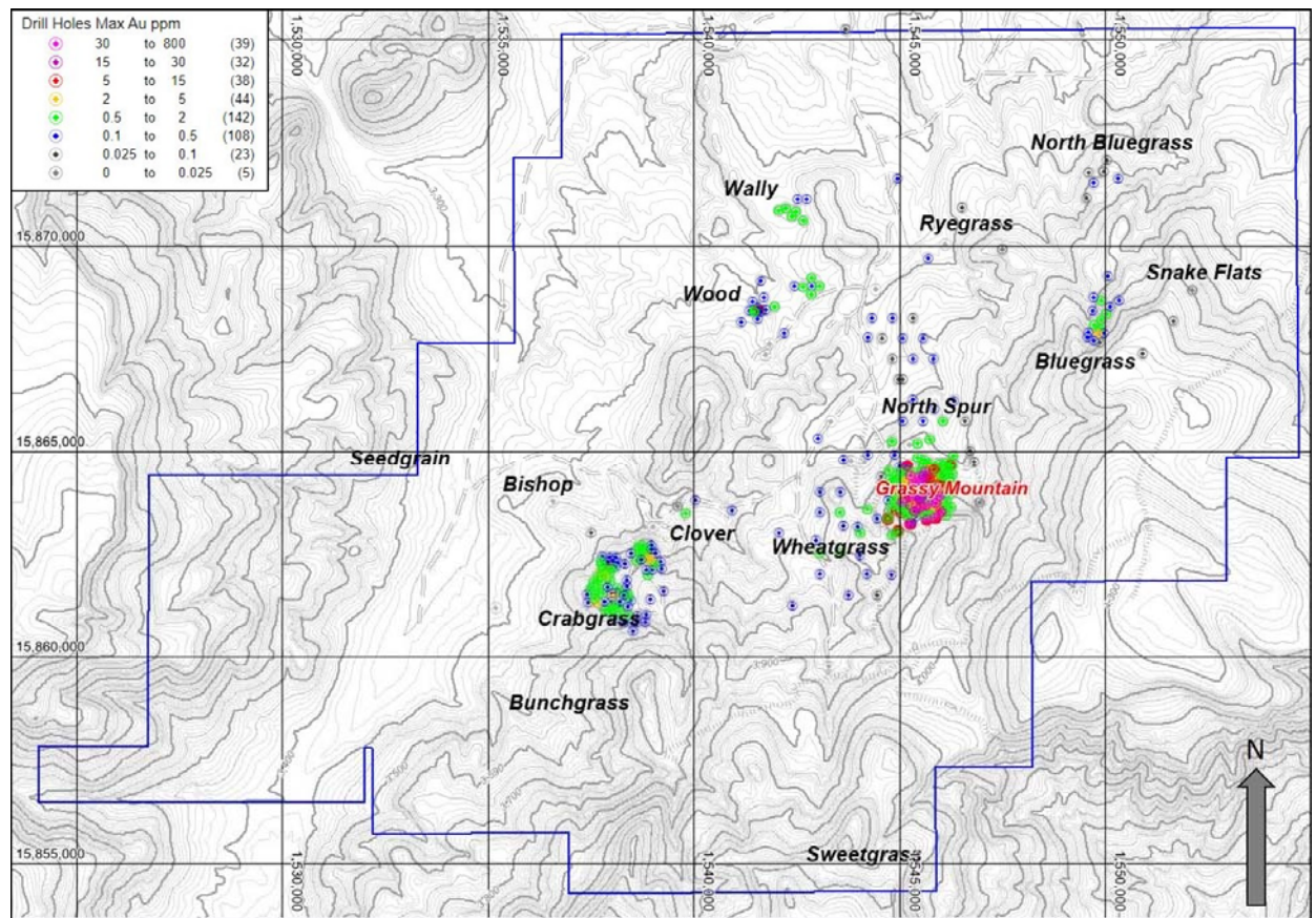
Figure 6-1: Outlying Target Area Map
