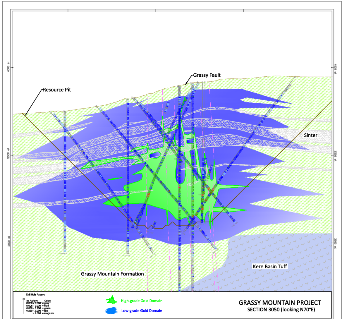
Figure 14-1: Cross Section 3050 Showing Gold Domains
