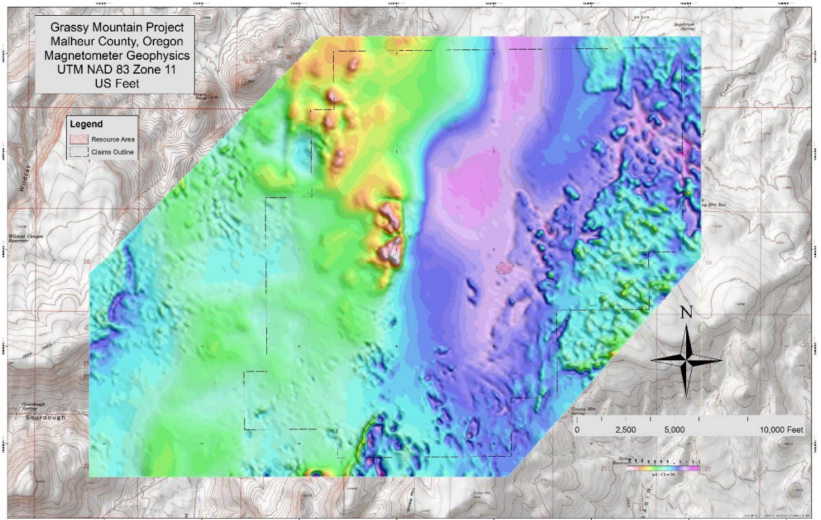
Figure 9-1: 2018 Aerial Magnetic Survey of Grassy Mountain Area
