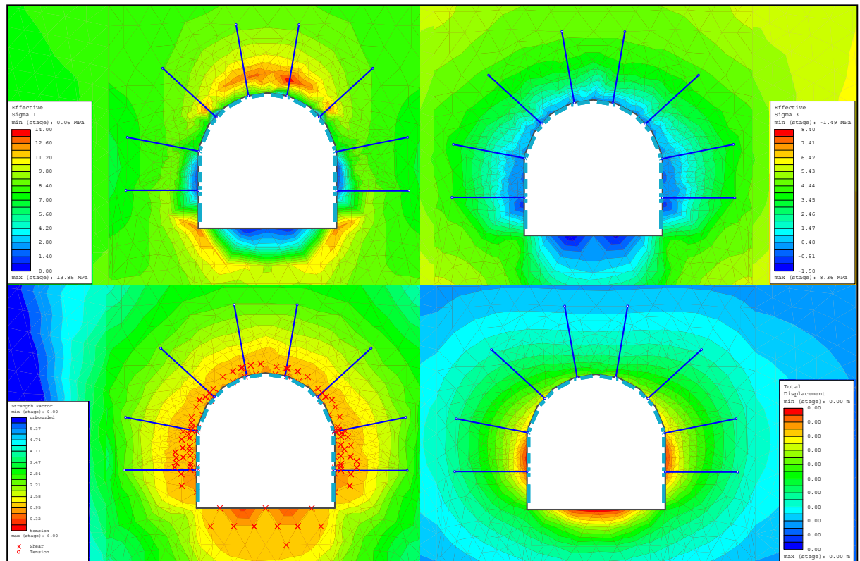
Figure 16-13: Modeling Results for Decline Ramp; a) Major Principal Stress, S1; b) Minor Principal Stress, S3; c) Strength Factor, SF; d) Displacements, D.
